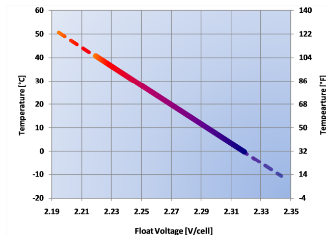
Fig. 6 : Recommended Float Voltage at different temperatures
