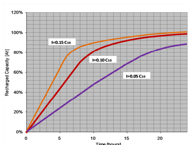
Fig. 7 : Recharge curves at 2.4 V/cell with different limit of current
