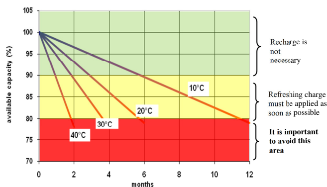
Fig. 8 : Storage time versus temperatures
